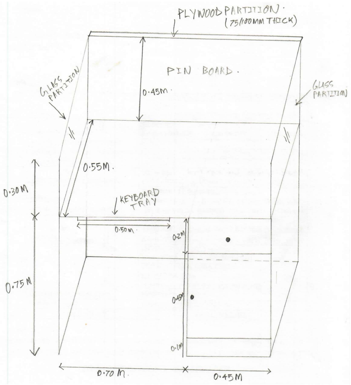
TYPICAL PLAN OF WORK-STATION
